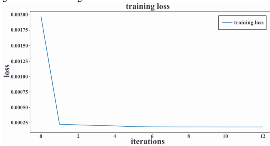
Figure 5. Training loss.
