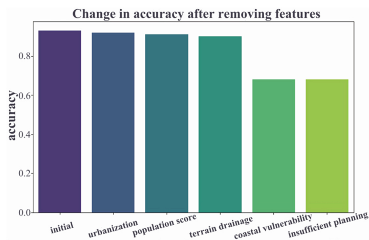
Figure 3. Sensitivity analysis result chart.
